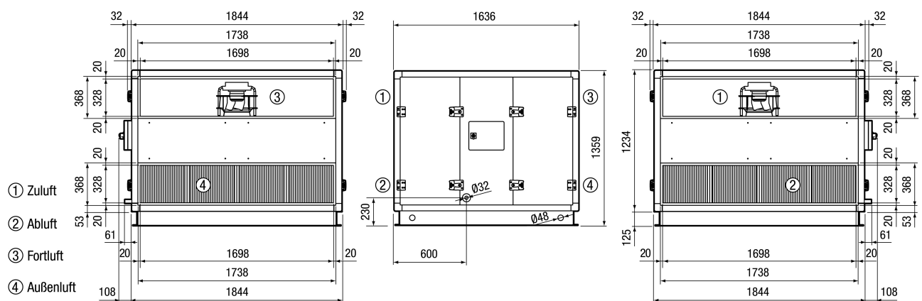
Reco-Boxx 4000 ZXR-L Linksversion
