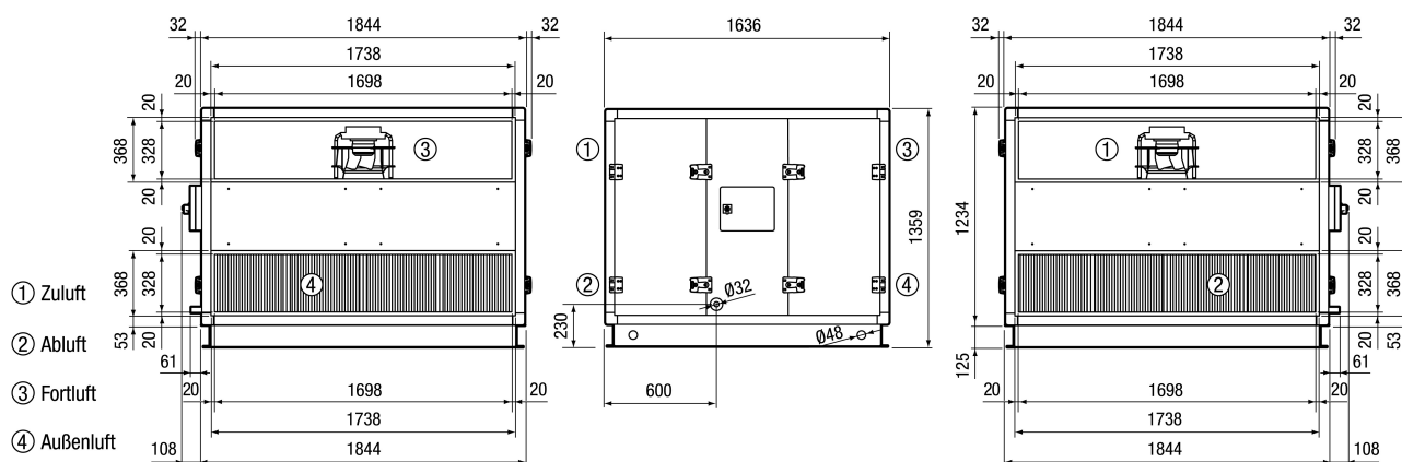
Reco-Boxx 4000 ZXR-L Linksversion
