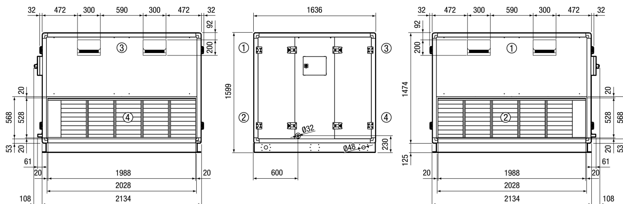
Reco-Boxx 5000 ZX-L Linksversion
