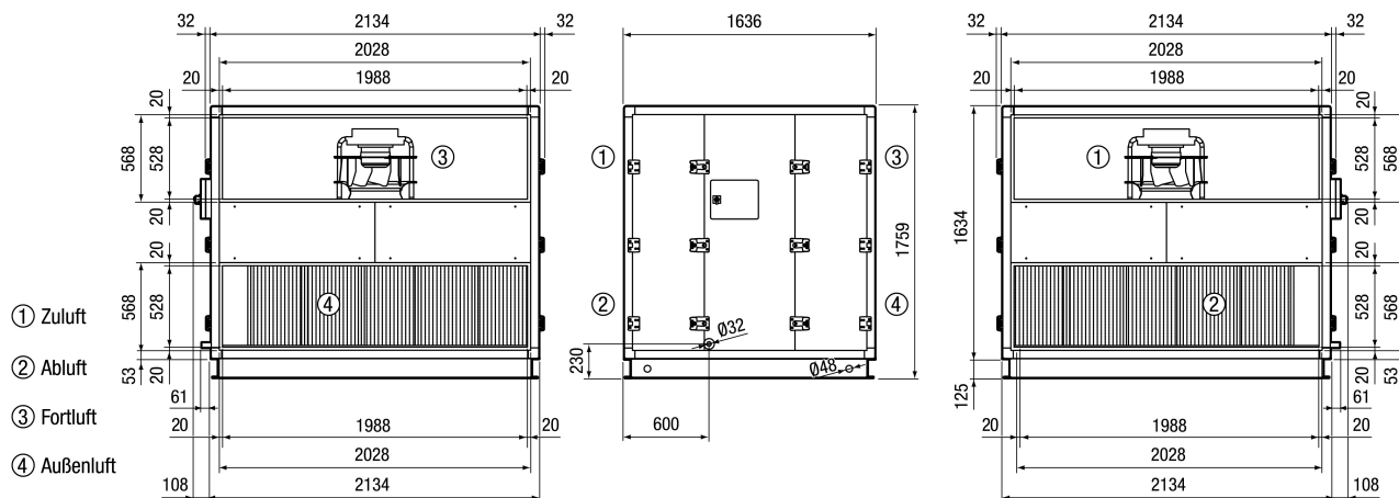
Reco-Boxx 5000 ZXR-L Linksversion
