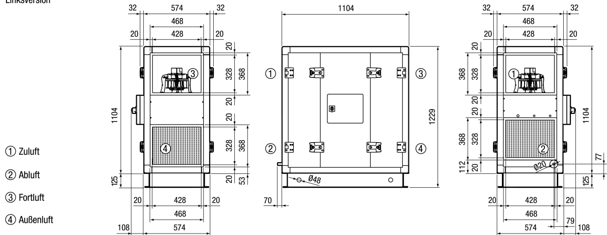
Reco-Boxx 800 ZXR-L Linksversion
