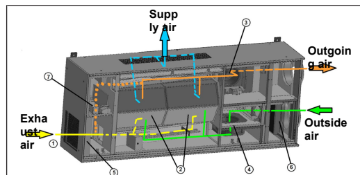
Illustration 1: Ventilation and air extraction, schematic diagram, geniovent.x 900 F R.
